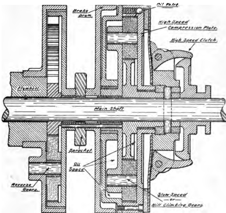
FIG. 262.—Section of Oldsmobile Two-Speed and Reverse Transmission.
